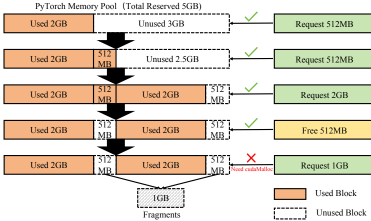
Fig. 17. GPU memory fragmentation in PyTorch's caching allocator.
