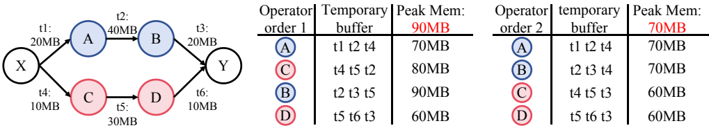
Fig. 18. Impact of operator execution order on temporary buffer and GPU memory peak.
