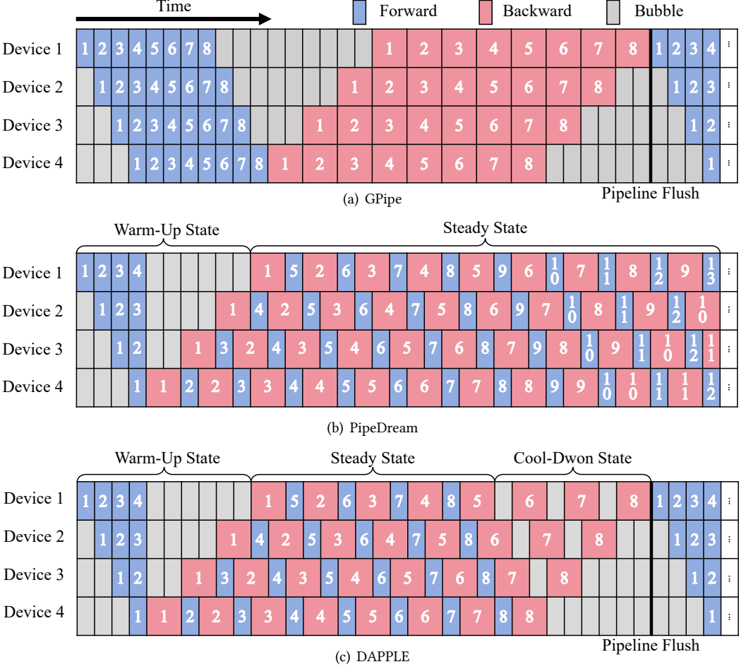
Fig. 15. Comparison of pipeline parallel scheduling strategies. To simplify the illustration, the backward propagation time is assumed to be twice the forward propagation time.
