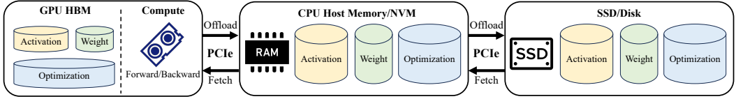
Fig. 5. Offloading system for DNN training.
