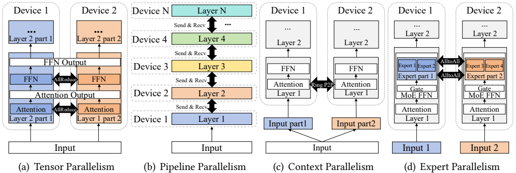
Fig. 13. Distributed training methods (Transformer examples). White and gray data represents replicas held by every device, while colorful data denotes unique data exclusive to individual devices. Notably, in EP, Input 1 and Input 2 are introduced by DP, which differs from the input partitioning in CP.
