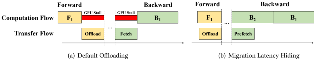
Fig. 6. Execution timeline comparison for offloading scheduling. (a) Default Offloading incurs GPU stalls that interrupt model computation; (b) Migration Latency Hiding mitigates stalls by parallelizing migration and computation.
