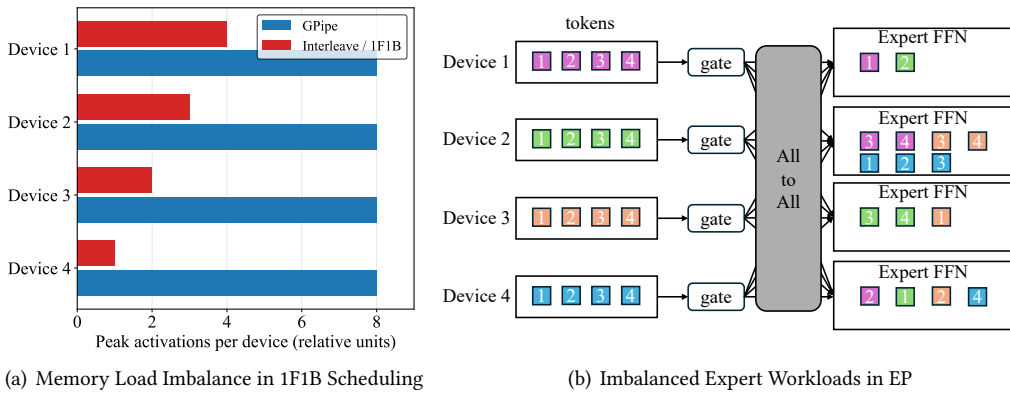
Fig. 16. Memory load imbalance in distributed training. (a) Memory load imbalance in 1F1B scheduling, where earlier pipeline stages have higher memory loads; (b) Memory load imbalance in EP caused by the random routing of tokens by the gating function.
