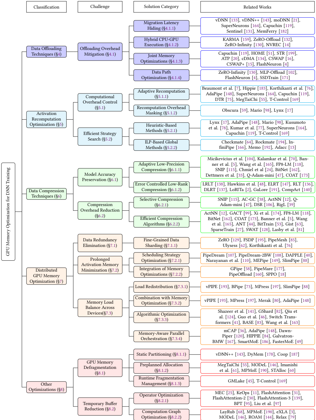
Fig. 4. Overview of memory optimization techniques
