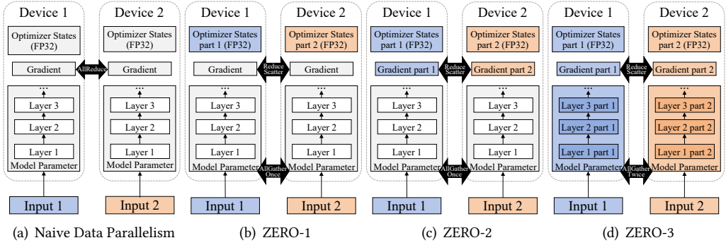
Fig. 14. Evolution of data redundancy elimination from data parallelism to ZeRO. White and Gray data represents redundant replicas held by every device, while colorful data denotes unique data exclusive to individual devices.
