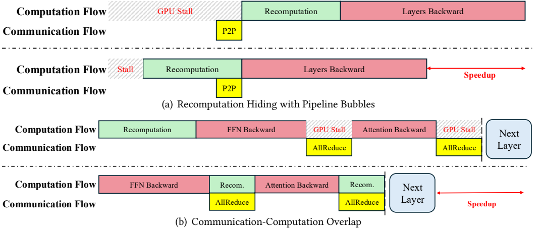
Fig. 9. Recomputation Overhead Masking. (a) Hiding the overhead of recomputation within the idle bubbles of pipeline scheduling; (b) Overlapping recomputation with communication operations. For each subfigure, the upper part presents the naive scheme, while the lower part shows the optimized scheme.
