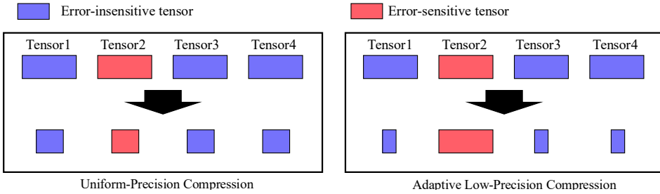
Fig. 11. Illustration of adaptive low-precision compression. Uniform-precision compression applies the same precision to all tensors, while adaptive low-precision compression assigns higher precision to error-sensitive tensors and lower precision to error-insensitive tensors.
