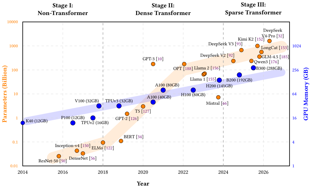
Fig. 3. Comparison of the growth trends in model parameter scales and GPU memory capacity.
