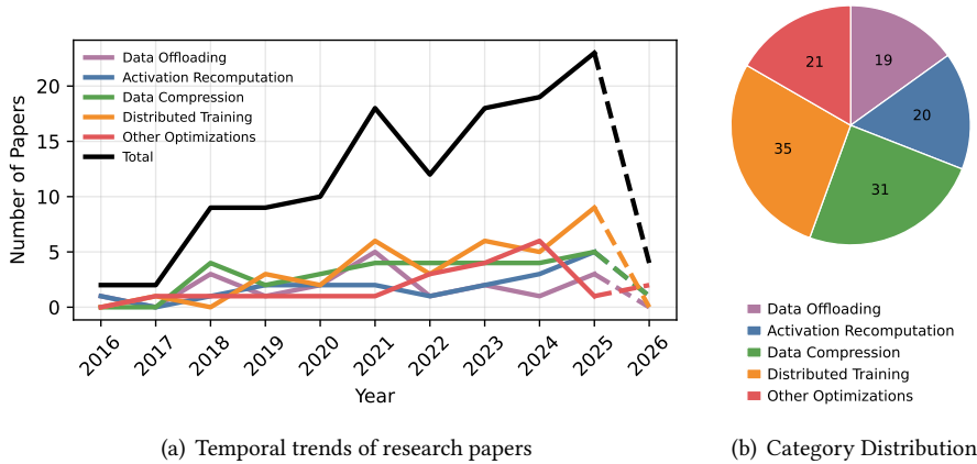
Fig. 1. Overview of research in GPU memory optimization for DNN training. (a) Temporal trends of research papers from 2016 to 2026 (dashed lines indicate partial data up to June 2026). (b) Distribution of the five research categories.
