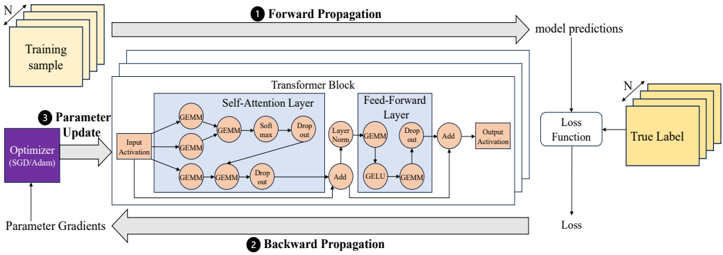
Fig. 2. Training workflow of DNNs.
