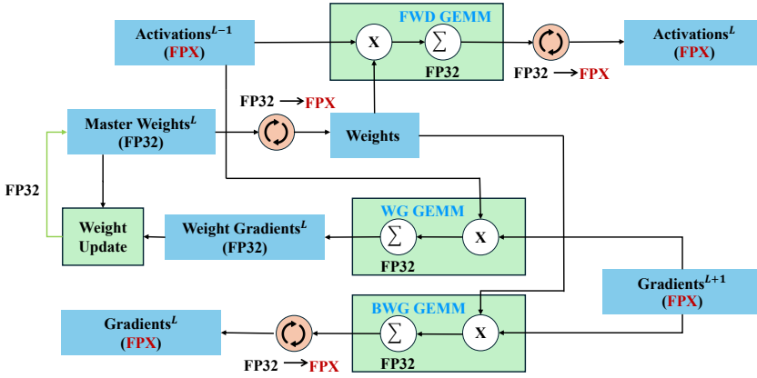
Fig. 12. Illustration of mixed precision training. Low precision is used for most forward and backward computations, while sensitive paths such as accumulation and parameter updates remain in higher precision.
