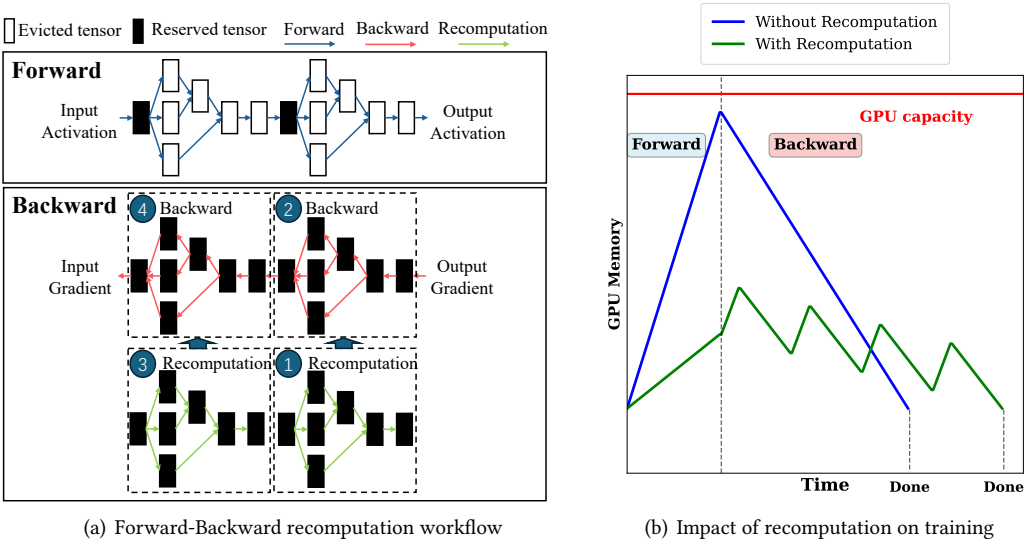
Fig. 8. Schematic illustration of activation recomputation and its impact on training. (a) Forward-Backward recomputation workflow; (b) Impact of recomputation on training. Recomputation reduces peak GPU memory consumption at the cost of introducing additional computational overhead.
