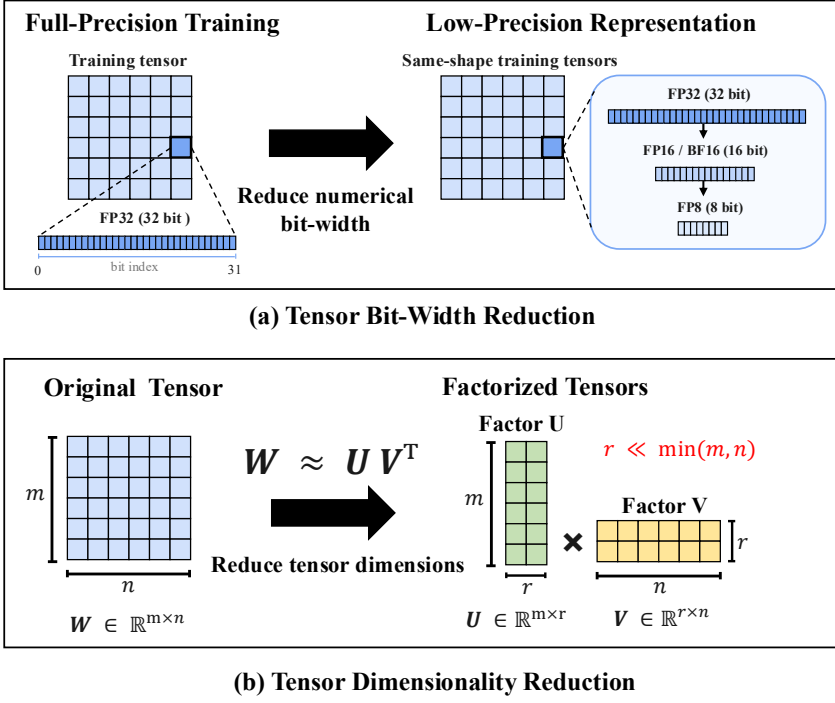
Fig. 10. Overview of data compression techniques for memory-efficient DNN training. Low-precision and low-rank training reduce memory usage by exploiting numerical precision redundancy and low-dimensional structure in training tensors.
