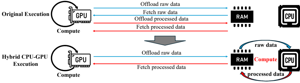
Fig. 7. Hybrid CPU-GPU Execution reduces the number of data migrations by scheduling computations directly on the CPU.
